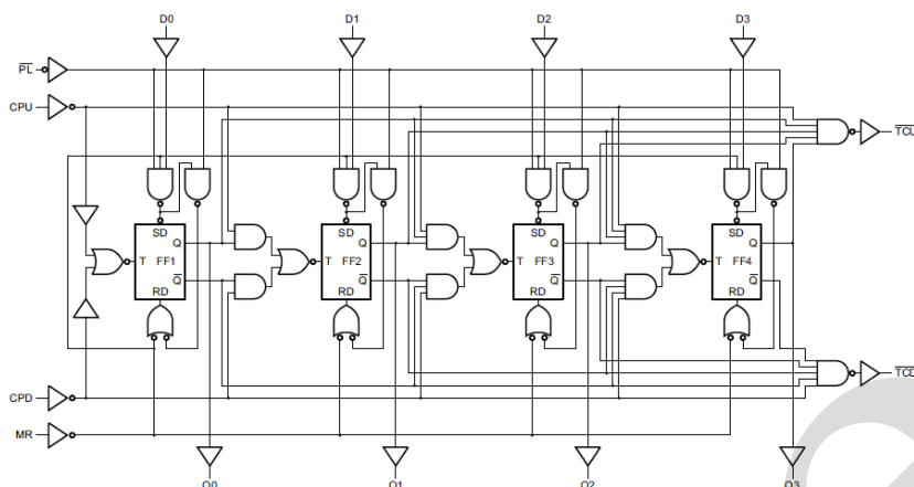
Figure 4. Logic diagram
